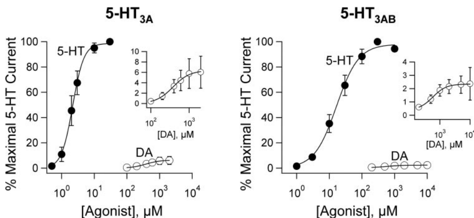
Fig. 1. 5-HT and DA concentration-response relationships for 5-HT 3A and 5-HT 3AB receptors, normalized to maximal 5-HT-evoked current responses. Note the low efficacy and potency of DA relative to 5-HT. Insets show DA concentration-response relationships with expanded scales to provide more detail. Data are expressed as mean \pm standard deviation ( n = 20 –48 for 5-HT 3A receptors and 4–18 for 5-HT 3AB receptors).
