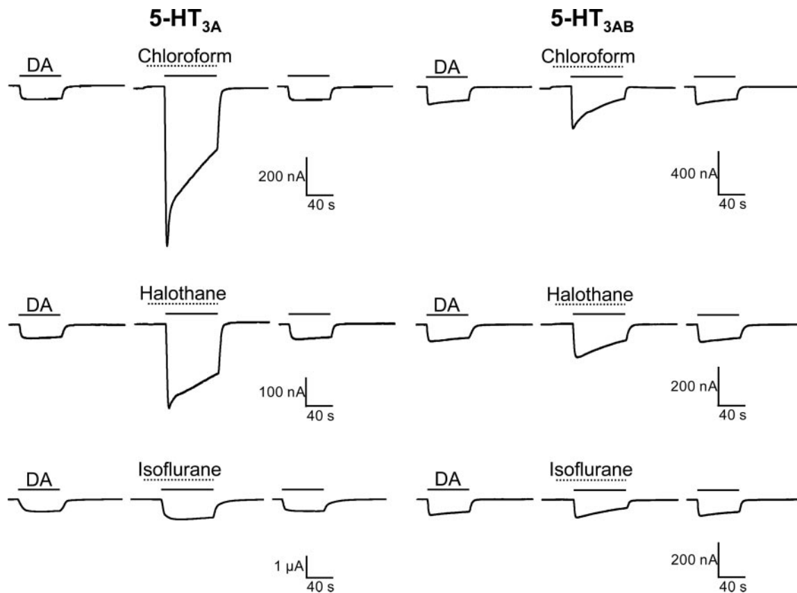
Fig. 2. Representative current traces illustrating the effects of 2 MAC chloroform, halothane, and isoflurane on current responses elicited by receptor-saturating concentrations of DA on 5-HT 3A and 5-HT 3AB receptors. The solid lines above the traces represent perfusion of the oocyte with DA, and the dotted lines represent perfusion with anesthetic. DA concentration was 1 mM for 5-HT 3A receptors and 2 mM for 5-HT 3AB receptors.
