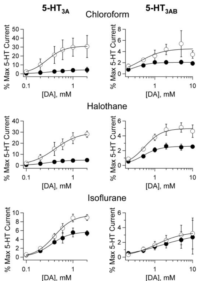
Fig. 4. DA concentration-response relationships for 5-HT 3A and 5-HT 3AB receptors in the absence and presence of 2 MAC chloroform, halothane, and isoflurane, normalized to maximal 5-HT-evoked current responses. Closed circles represent controls (i.e., current responses evoked by DA alone), and open circles represent current responses evoked by DA in the presence of anesthetic. The controls were matched (i.e., the same oocytes were used for experiments with and without anesthetic). Note the different scales on the vertical axes for 5-HT 3A and 5-HT 3AB receptors. Data are expressed as mean \pm standard deviation ( n = 3-6 ).
